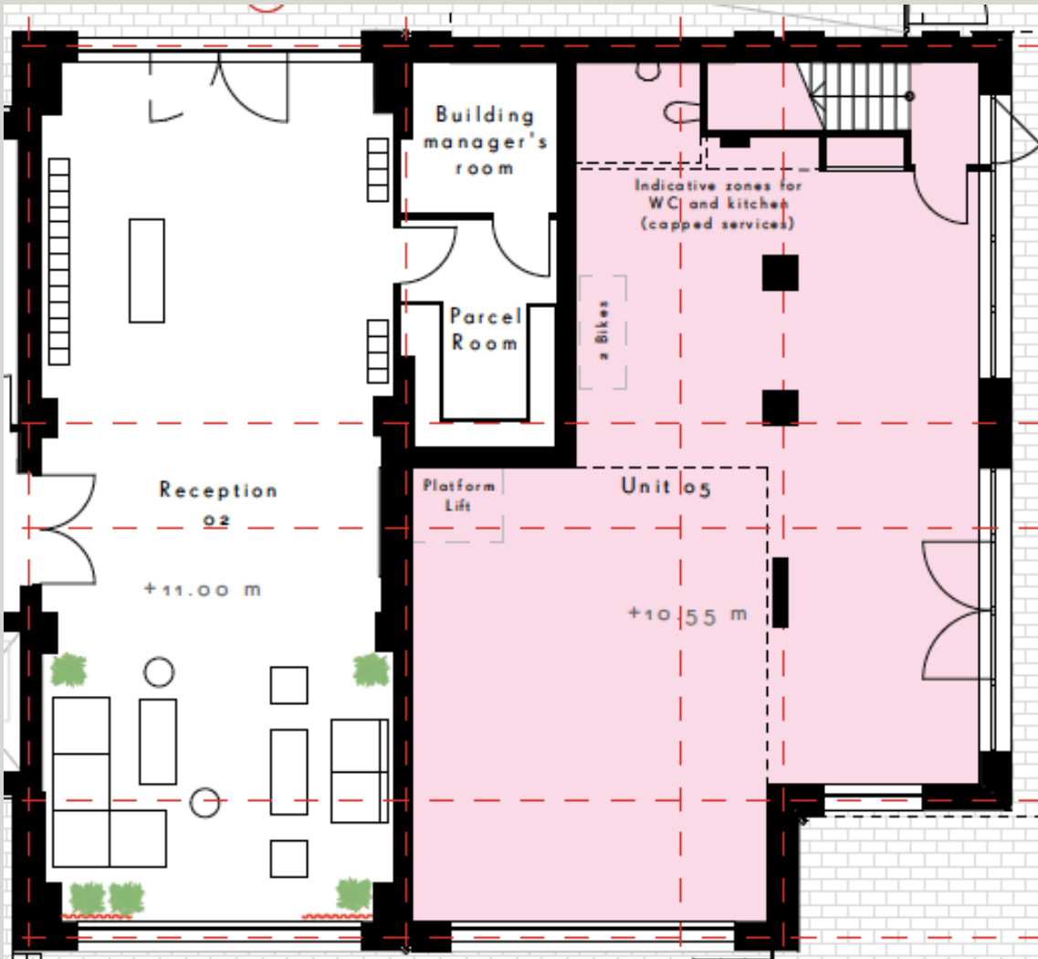
Ground Floor
