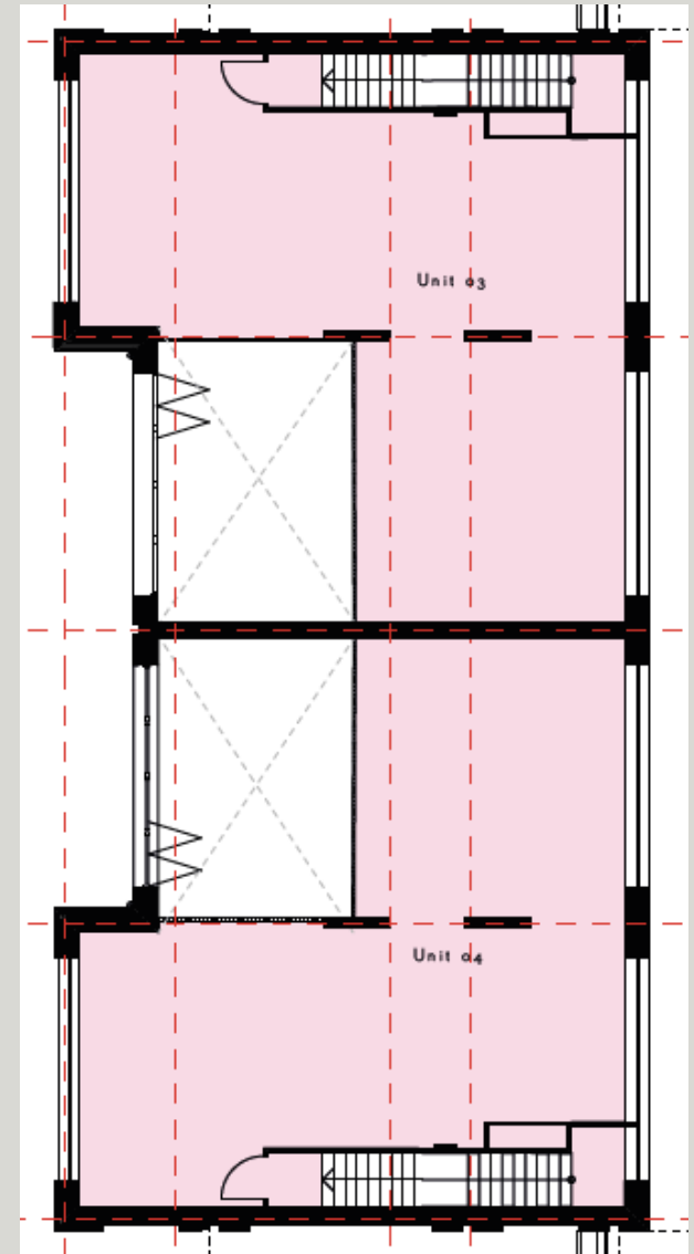
Mezzanine Floor
